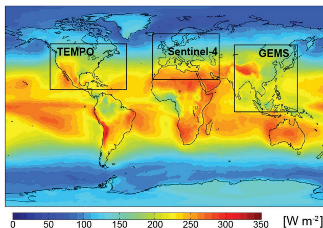
Figure 2: MERRA 2006-2007 all-sky incident solar radiation overlaid with sampling domains of planned GEO Earth observation platforms.
