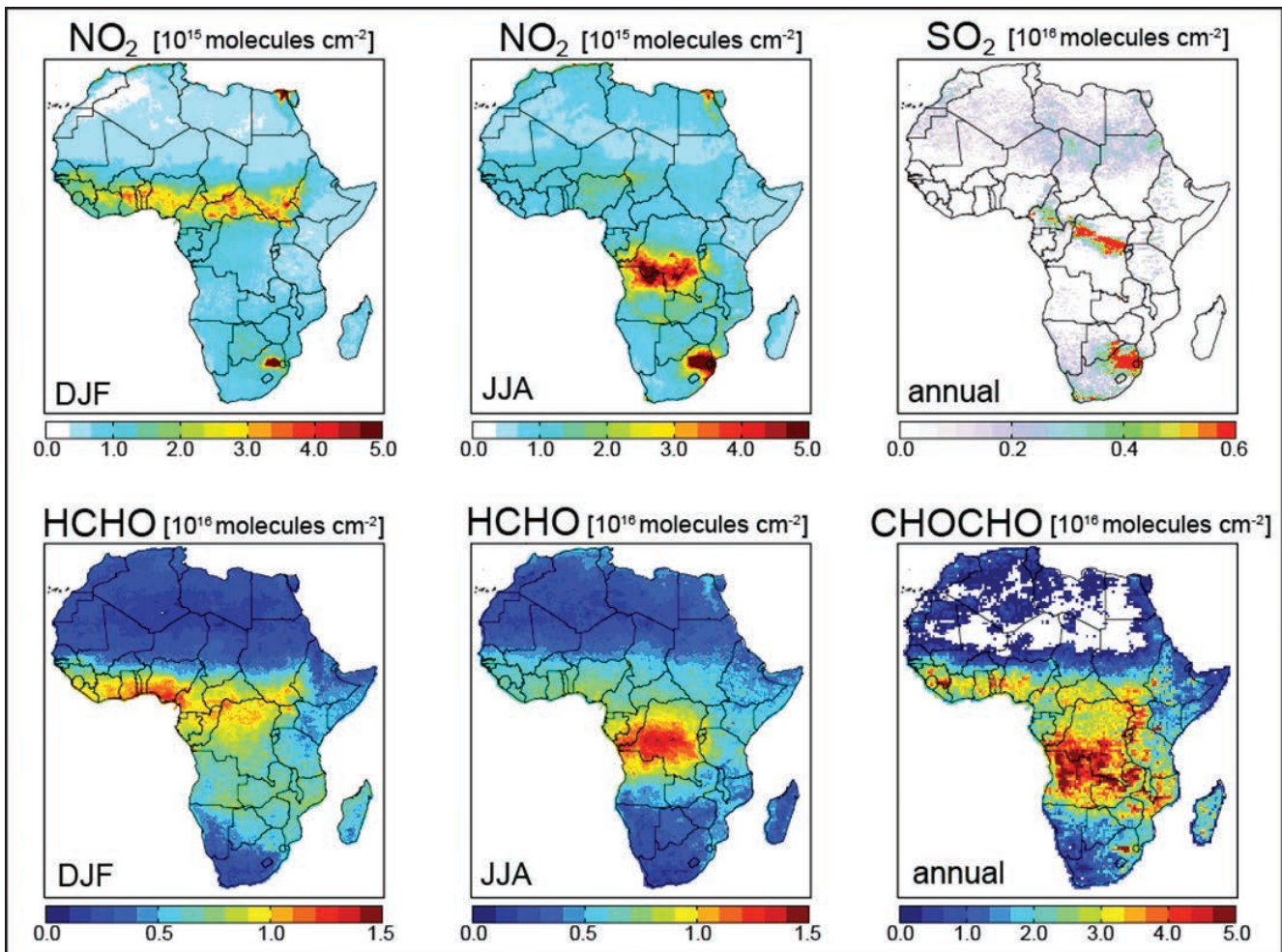
Figure 1: Mean concentrations of tropospheric nitrogen dioxide (NO 2 ), PBL-weighted sulfur dioxide (SO 2 ), and total column formaldehyde (HCHO) and glyoxal (CHOCHO) from OMI for 2006-2007.
